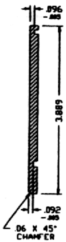
SECTION E-E
